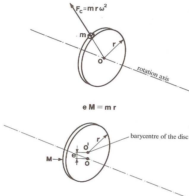
Fig. 1 - Centrifugal force generated by an unbalance or by an eccentricity.
